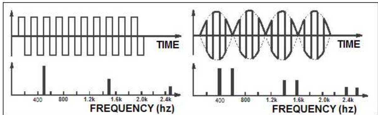
Figure 2-21: A square wave being ring modulated by a sine wave.
