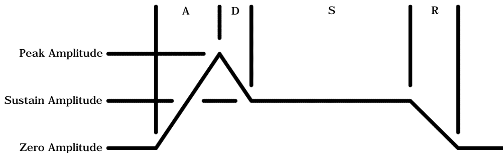
Figure 4-1 ADSR Envelope.
