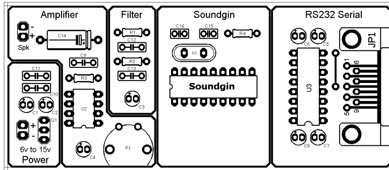
Parts Layout
