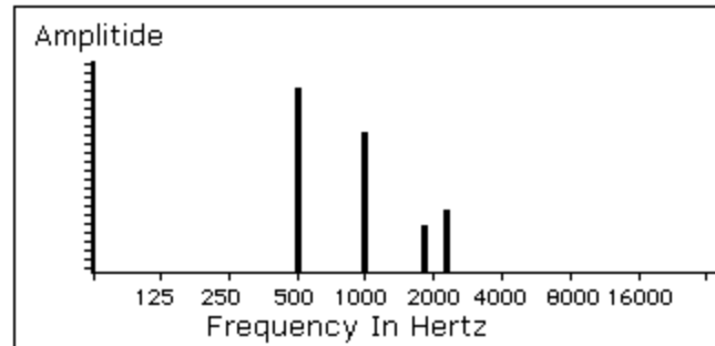
Figure 2-3: A Spectrograph.
