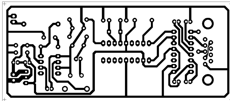
Board Traces.
