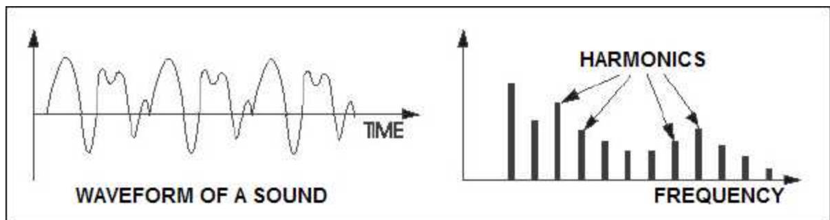
Figure 2-2: The waveform and spectrum of a complex sound.
