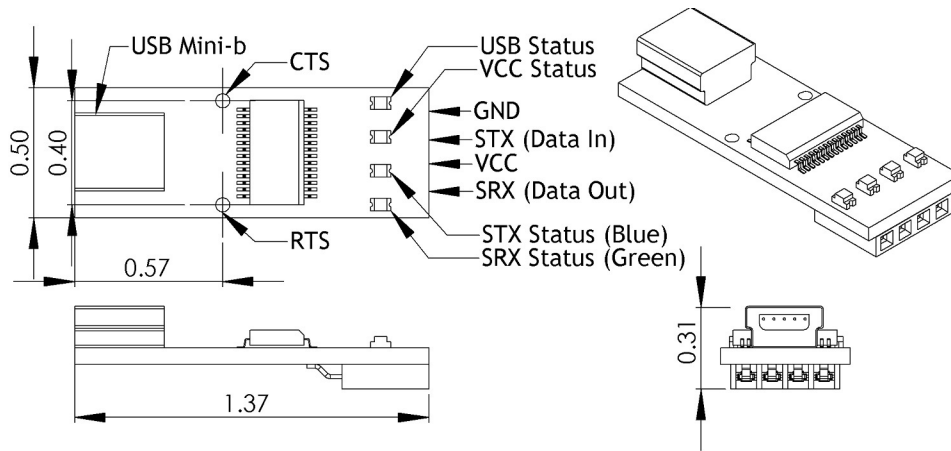
S27-USB-SERIAL Pinout
