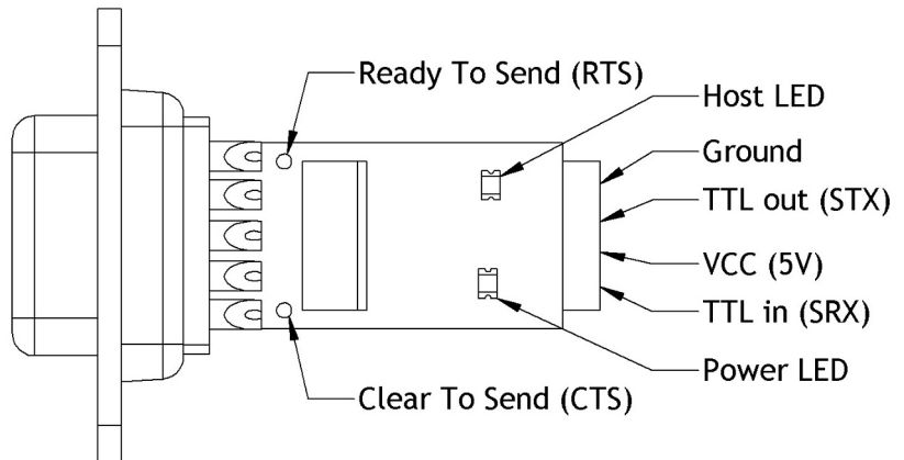
Pin Out Diagram
