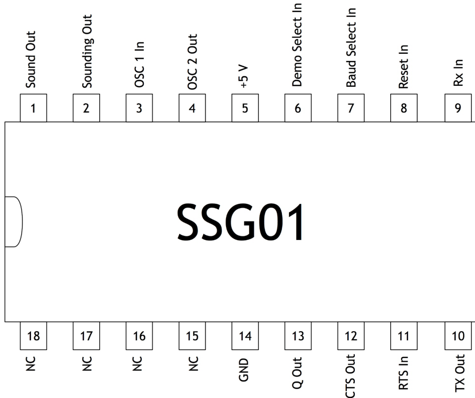
Pinout Diagram
